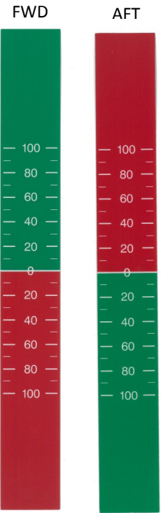
Propulsion scales
